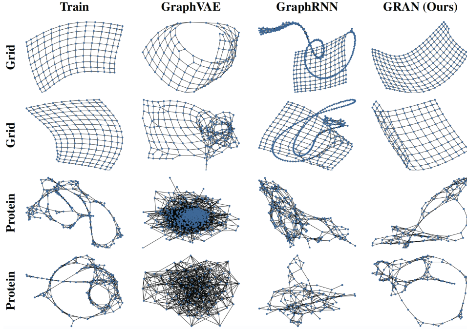
Figure 9.3: Examples of graphs generated by a basic graph-level VAE (Section 9.1), as well as the GraphRNN and GRAN models. Each row corresponds to a different dataset. The first column shows an example of a real graph from the dataset, while the other columns are randomly selected samples of graphs generated by the corresponding model [Liao et al., 2019a].
