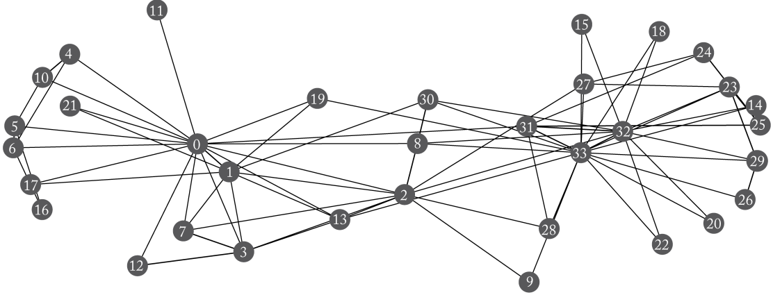
Figure 1.1: The famous Zachary Karate Club Network represents the friendship relationships between members of a karate club studied by Wayne W. Zachary from 1970–1972. An edge connects two individuals if they socialized outside of the club. During Zachary’s study, the club split into two factions—centered around nodes 0 and 33—and Zachary was able to correctly predict which nodes would fall into each faction based on the graph structure [Zachary, 1977].
