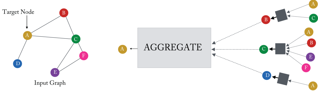
Figure 5.1: Overview of how a single node aggregates messages from its local neighborhood. The model aggregates messages from A’s local graph neighbors (i.e., B, C, and D), and in turn, the messages coming from these neighbors are based on information aggregated from their respective neighborhoods, and so on. This visualization shows a two-layer version of a message-passing model. Notice that the computation graph of the GNN forms a tree structure by unfolding the neighborhood around the target node.
