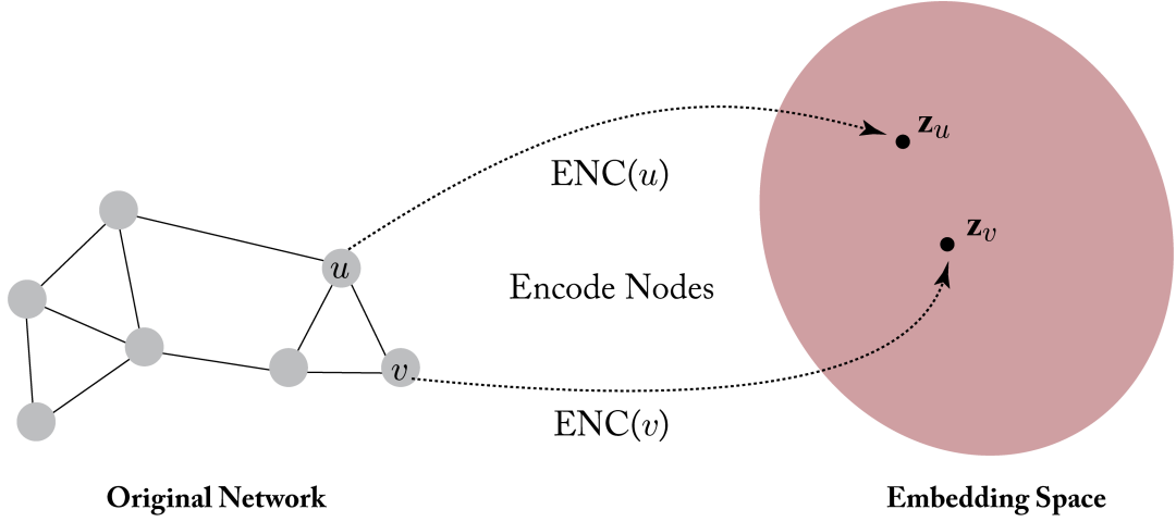
Figure 3.1: Illustration of the node embedding problem. Our goal is to learn an encoder ( \text{ENC} ), which maps nodes to a low-dimensional embedding space. These embeddings are optimized so that distances in the embedding space reflect the relative positions of the nodes in the original graph.
